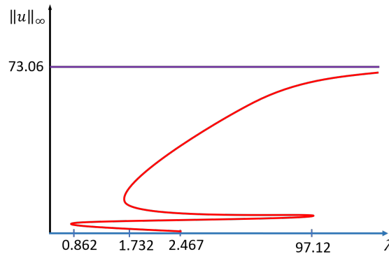
FIGURE 8. An approximate bifurcation diagram of positive solutions for (14) when \gamma = 1 ; K = 75 ; c = 1.89 , m = 1000 .
